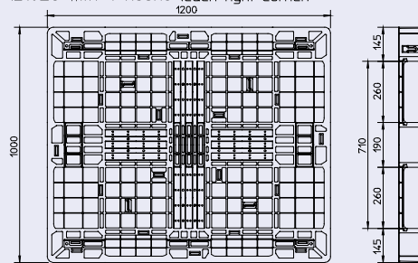
EXA-1210EU with 4 hooks (each right corner)
