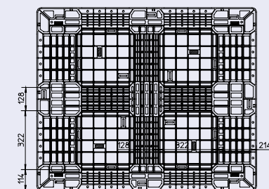
EXA-1210EU with 4 hooks (each right corner)
